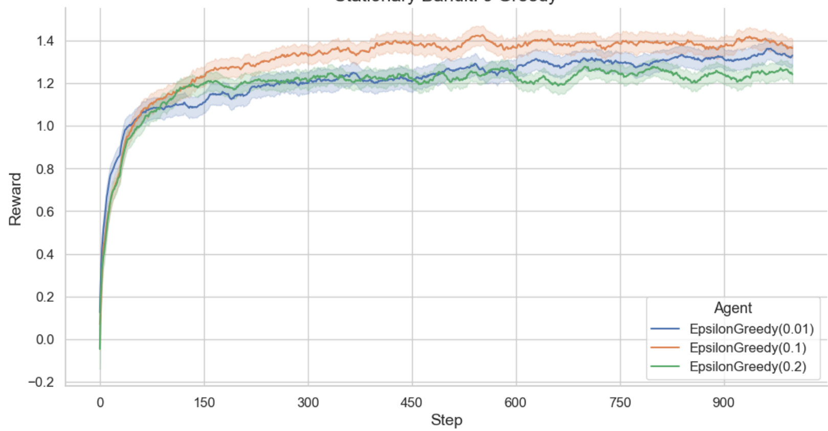
Stationary Bandit: \epsilon -Greedy
